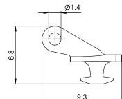
180° Front hinge 180度钉铰 (平铰)
