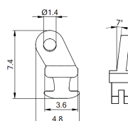
90 °Front hinge with inclination 带倾角的90度前铰
