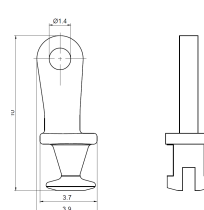
High Male Hinge 高腰阳钉铰 90°
