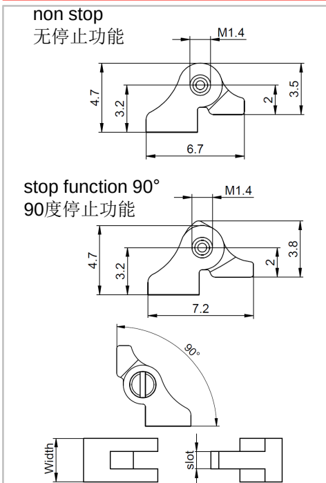
Profile: C stainless steel - 不锈钢C型
